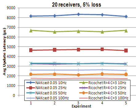
Fig. 19. ISISlab: 20 readers, 5% loss
