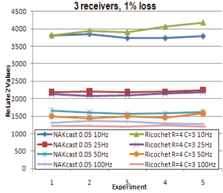
Fig. 14. ISISlab: 3 readers, 1% loss
