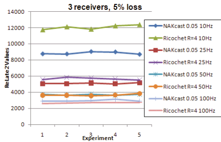
Fig. 16. ISISlab: 3 readers, 5% loss
