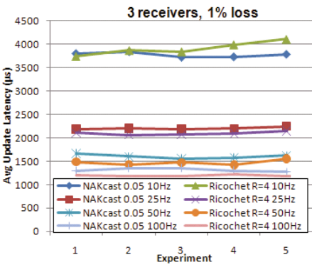
Fig. 13. ISISlab: 3 readers, 1% loss
