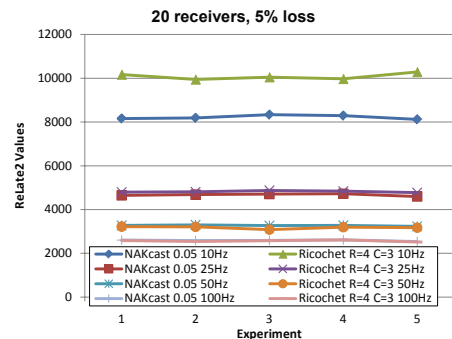
Fig. 20. ISISlab: 20 readers, 5% loss
