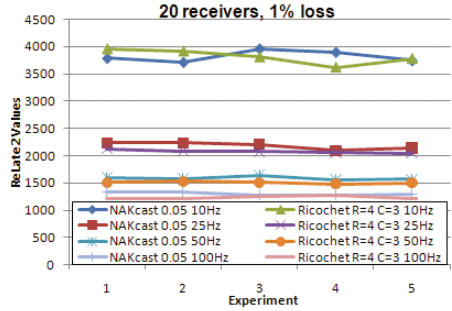
Fig. 18. ISISlab: 20 readers, 1% loss
