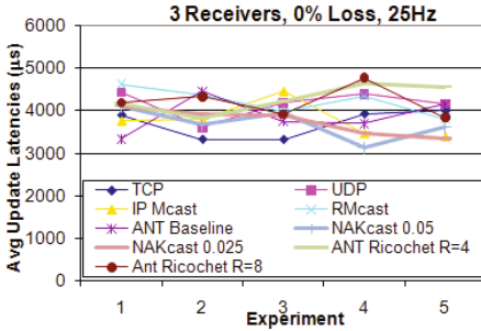
Fig. 7. Emulab: 3 readers, 0% loss, 25Hz
