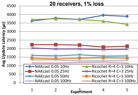
Fig. 17. ISISlab: 20 readers, 1% loss
