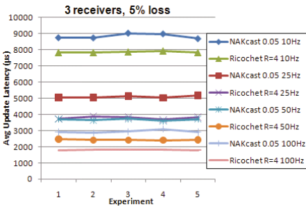
Fig. 15. ISISlab: 3 readers, 5% loss
