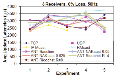
Fig. 8. Emulab: 3 readers, 0% loss, 50Hz
