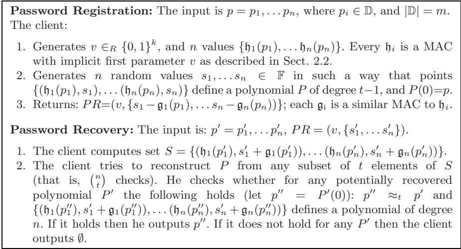
Fig. 2. Local Password Recovery
