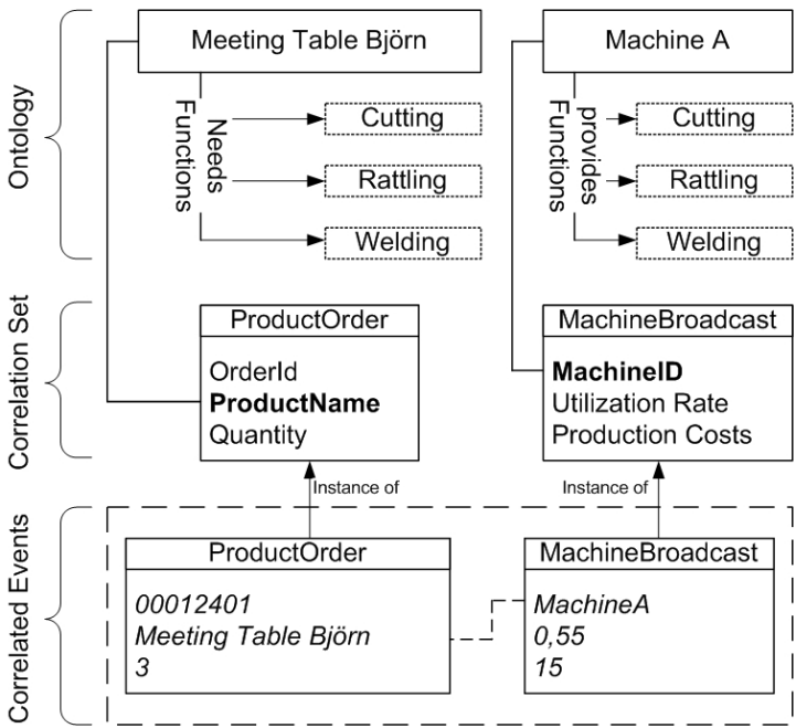
Fig. 2. Relation-based semantic correlation
