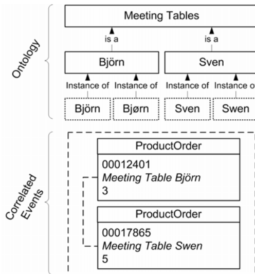
Fig. 1. Inherited semantic correlation
