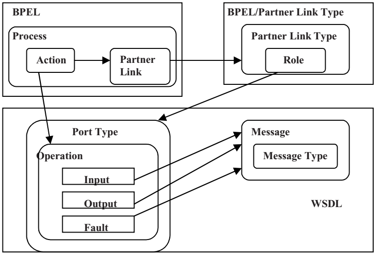
Fig. 2. Relation mapping between the BPEL process and the WSDL
