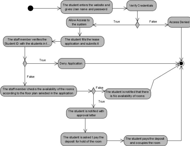
Fig. 6. Activity Diagram in VP – UML for Lease approval process
