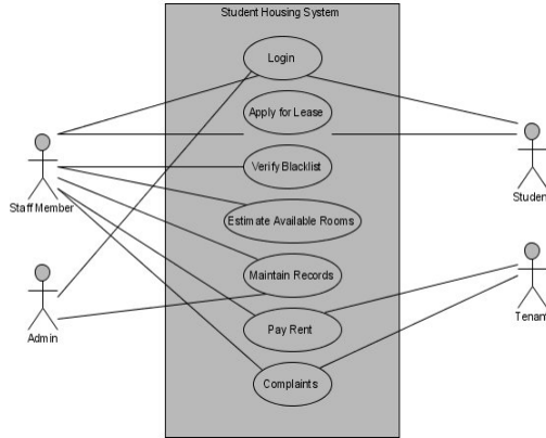
Fig. 5. Use case Diagram generated from VP – UML
