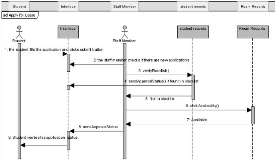
Fig. 7. Sequence Diagram in VP – UML for Lease approval business process
