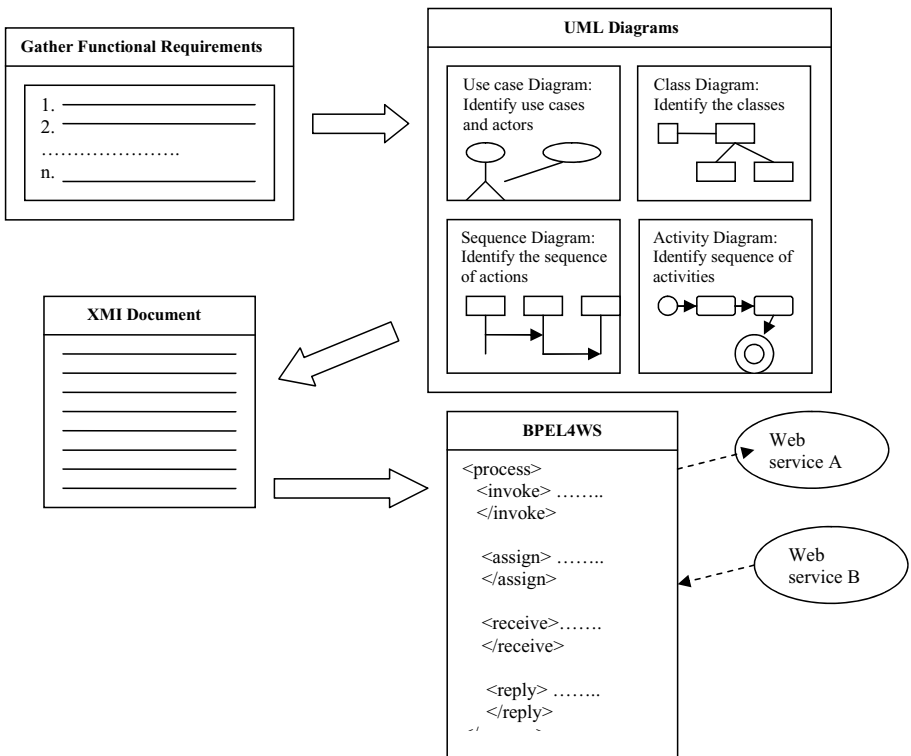
Fig. 3. The methodology for transforming UML Functional Requirements into BPEL Specification
