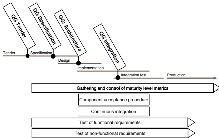
Fig. 1. Quality gates in context [17]
