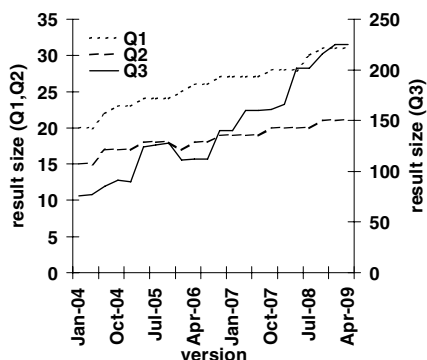
Fig. 6. Number of result items, Q1, Q2, Q3 for GO:0007610
