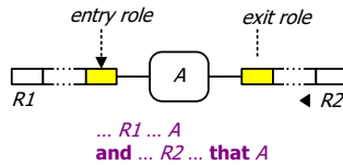
Fig. 9. A third pattern for verbalizing inner joins
