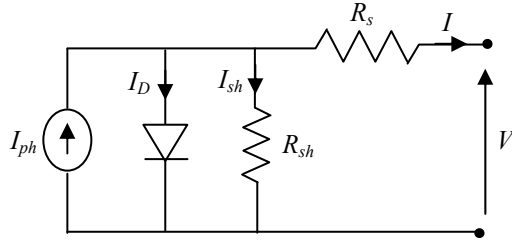
Fig. 1. Panel circuit model
