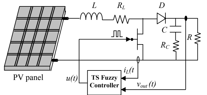
Fig. 5. Bloc diagram of the TS fuzzy controller
