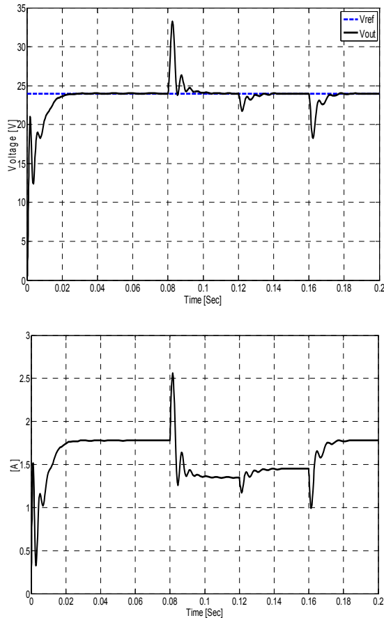
Fig. 8. Voltage and current response of the PI controlled boost converter subject to the same input voltage changing.
