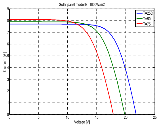
Fig. 3. LC120-12P PV module current – voltage curve when the temperature is 25, 50 and 75 ^{\circ}C .
