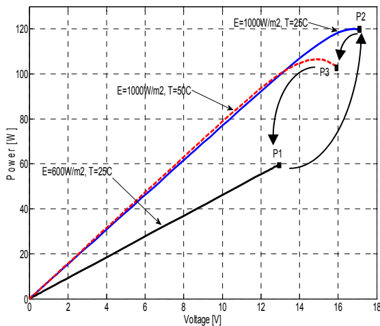
Fig. 6. The input voltage changing: P_1 \rightarrow P_2 \rightarrow P_3 \rightarrow P_1 , owing to the solar irradiation and cell temperature variation
