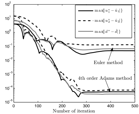
Fig. 2. Maximum errors of control and disturbance variables depending on the number of iterations for first (Euler method) and fourth order Adams method.
