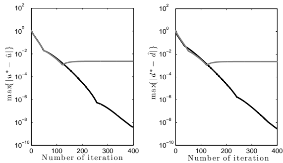
Fig. 1. Maximum errors of control and disturbance variables depending on the number of iterations for first (grey line) and fourth (black line) order Adams method.
