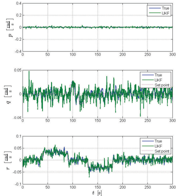
Fig. 5. The angular rates of rotation (\hat{p}, \hat{q}, \hat{r}) estimated by the SP-UKF using the Infante model dynamics during a maneuver presented in fig. 7.
