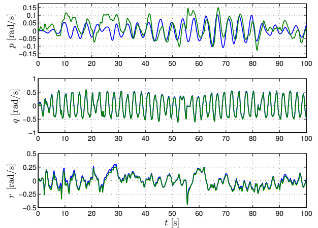
Fig. 9. The angular rates of rotation (\hat{p}, \hat{q}, \hat{r}) estimated by the SP-UKF using the CETUS II model dynamics during a maneuver presented in fig. 11.
