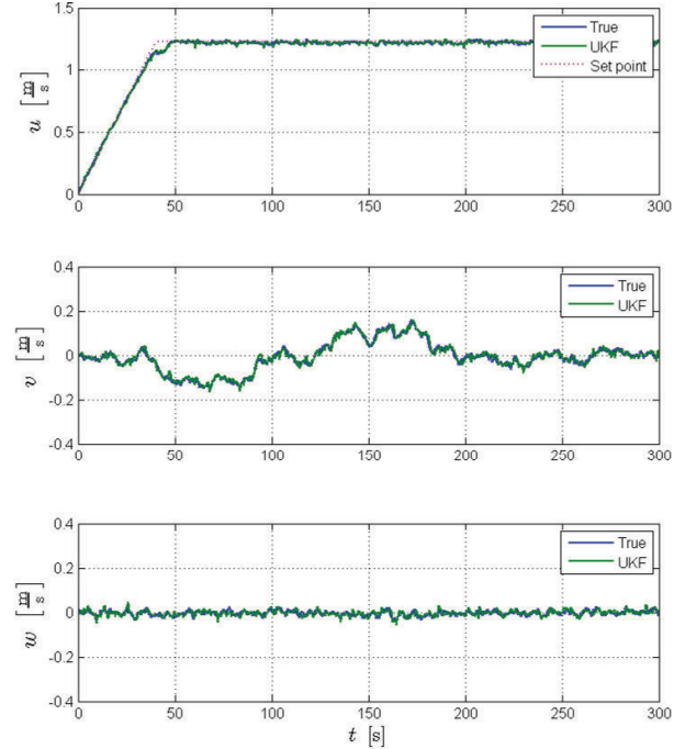
Fig. 4. The comparison of the original (incl. process noise) and SP-UK-filtered estimates of the (\hat{u}, \hat{v}, \hat{w}) – linear 3D speed-over-ground states based on the DVL measurements during the simulated composite maneuver of the Infante model dynamics presented in fig. 7.
