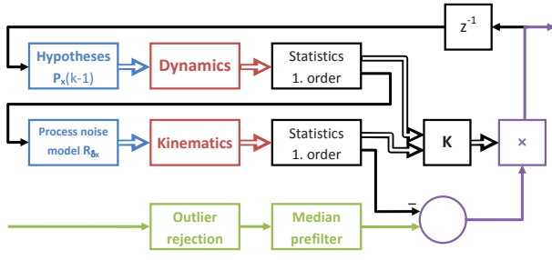
Fig. 1. Sigma-point Scaled Unscented Transform Kalman filter – SP-UKF.
