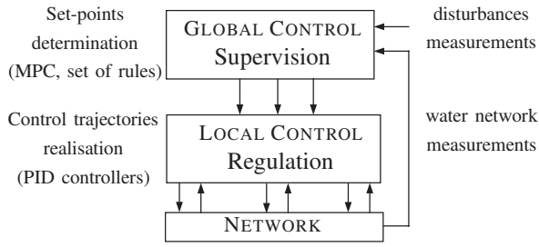
Fig. 1. Hierarchical structure for a water transport network
