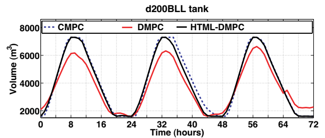
Fig. 10. Volume behaviour of d200BLL tank
