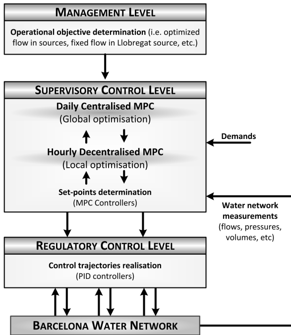
Fig. 2. HTML-DMPC structure
