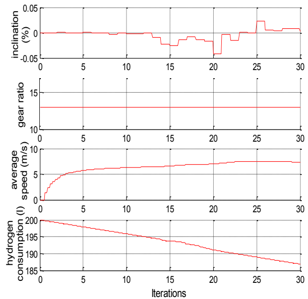
Figure 6: Test case 2: Constant gear ratio in real track
