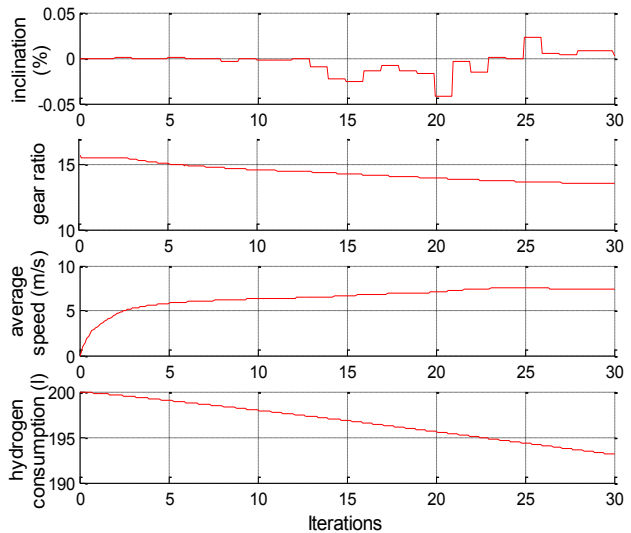
Figure 7: Test case 2: Variable transmission in real track
