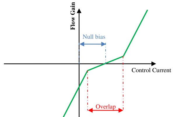
Fig. 3 : Flow Gain curve and main features
