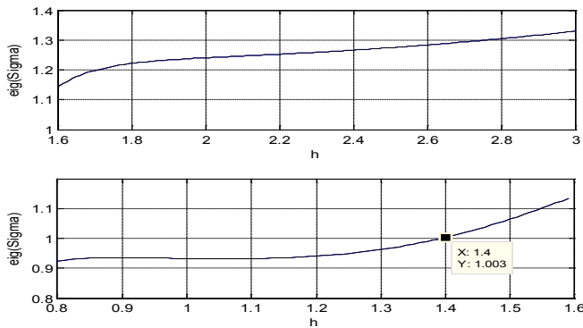
Fig. 5. \tau=1.6 seconds. Eigenvalue of \Sigma with largest magnitude for \tau < h (top) and for h < \tau < 2h (bottom).
