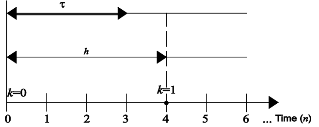
Fig. 3. Representation of the small delay case and the involved parameters for discrete-time systems. In this example h=4 and \tau=3 < h .
