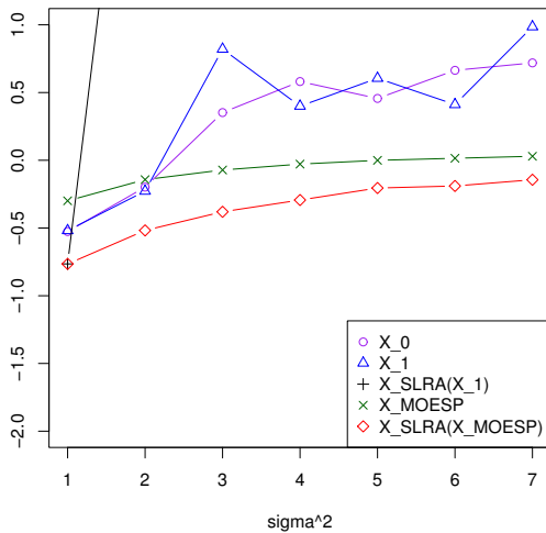
Fig. 4. Dependence of \log_{10}(RMSE) on \sigma^2
