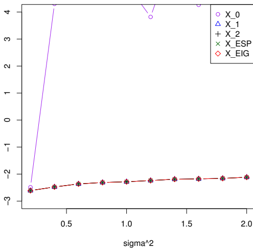
Fig. 1. \log_{10}(RMSE) for the estimates depending on the noise variance
