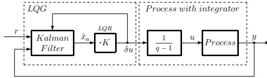
Fig. 7: Interconnection between the plant and the LQG controller.
