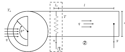
Fig. 1: Scheme of air heating system.
