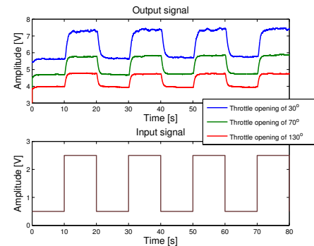
Fig. 2: System response to square wave input signal for the three throttle openings and sample period of 1\text{ ms} .
