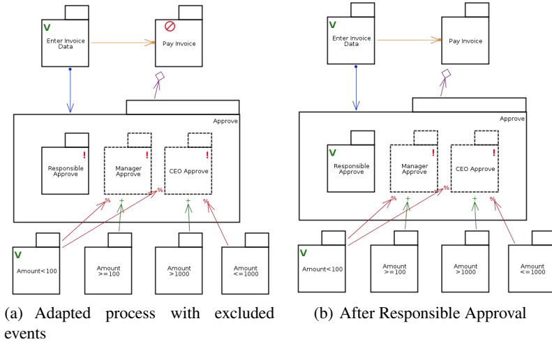
Fig. 2. Example of nested events and dynamically included and excluded events
