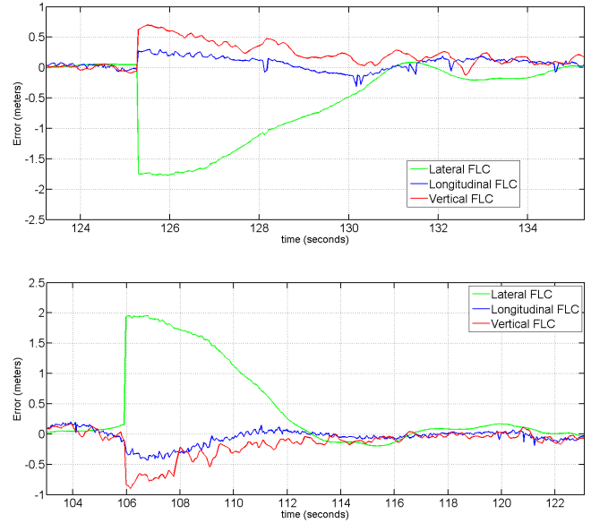
Fig. 17. Two tests of the response of the three controllers changing the code to inspect.
