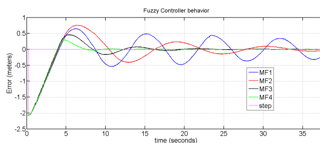
Fig. 8. Response of the different lateral speed controllers during the tuning phase of the inputs' range adjustment.
