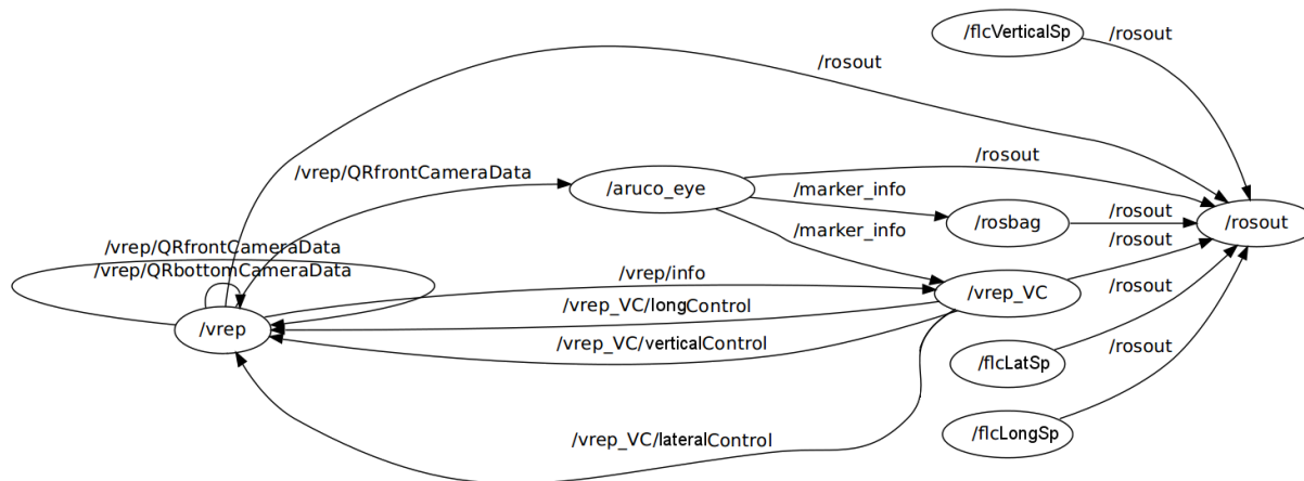
Fig. 6. Interaction between all the active processes from V-REP and ROS during the simulator tests.
