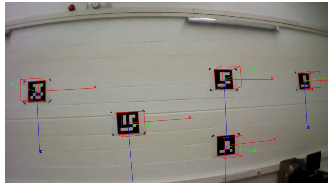
Fig. 14. Real image from the UAV camera processed using the ROS package of the ArUco library.
