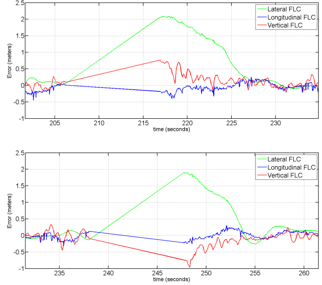
Fig. 16. Two tests of the response of the three controllers working in parallel against disturbances in the three axis.
