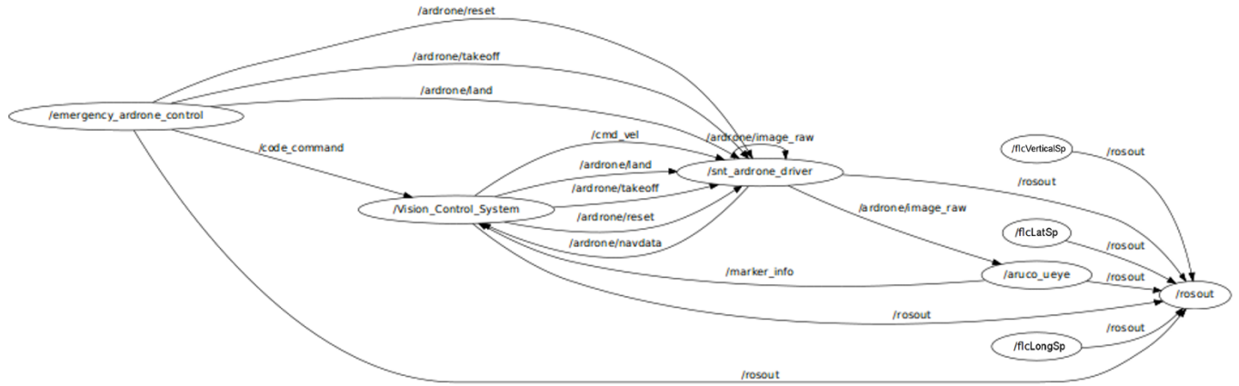
Fig. 12. Interaction between all the active processes of ROS during the real tests.
