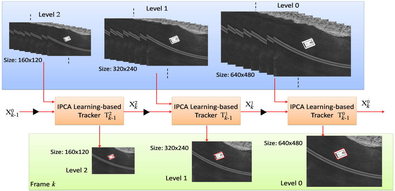
Fig. 3: Our visual tracker. The observation images up to k th frame are downsampled to create the MR structure. The motion model estimated in each level is used as the initial estimation of motion for next higher resolution image, leading to a higher tracking speed, better accuracy than a single full resolution-based tracking. The symbol \blacktriangleright is the recursion operator.
