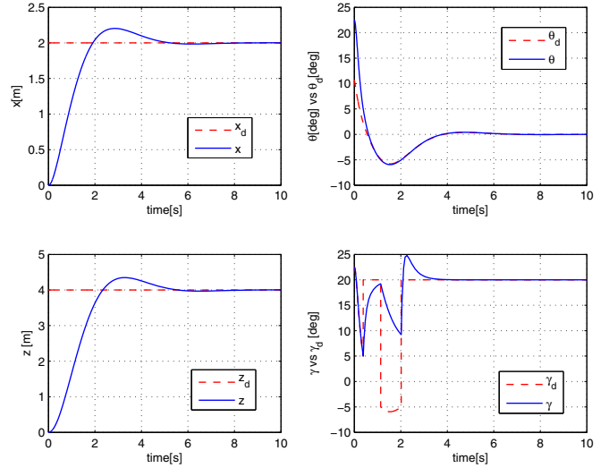
Fig. 6. States evolution: [left] Translational states and [right] rotational states
