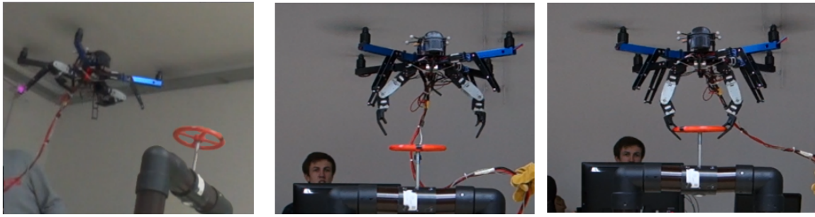
Fig. 6. MMUAV approaching and grabbing a valve: Taking off with arms stowed away for safety; approaching the valve; grabbing the valve.
