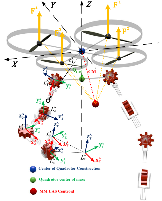
Fig. 2. Proposed UAS model showing quadrotor and manipulators (links expanded for clarity). 4 DOFs are shown for each arm to indicate a complete arm design [16].
