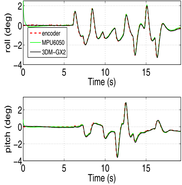
Fig. 2. Attitude estimation
