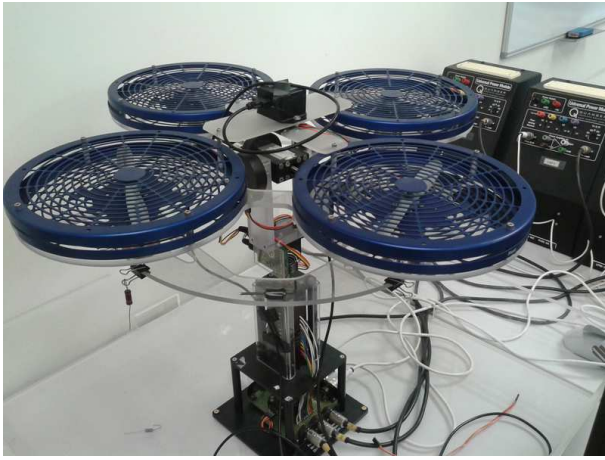
Fig. 1. Experimental platform
