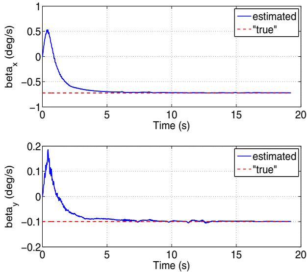
Fig. 3. Bias estimation
