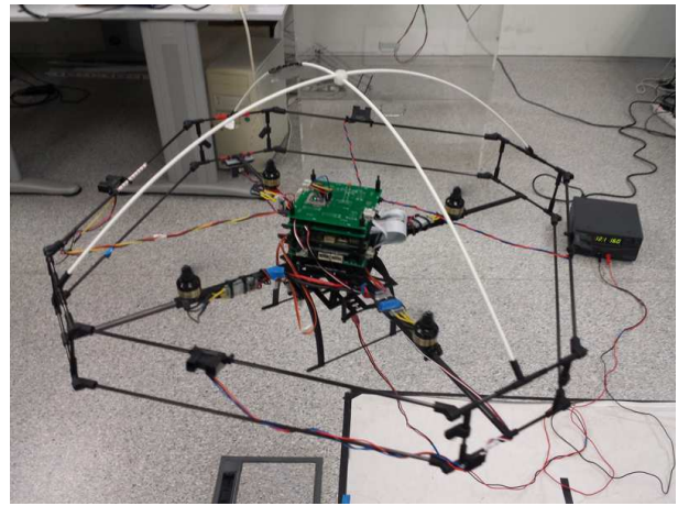
Fig. 5. Quadrotor prototype
