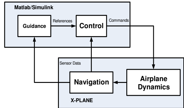
Figure 13. SIL Architecture
