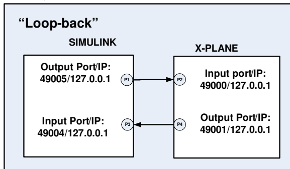
Figure 3. UDP Ports
