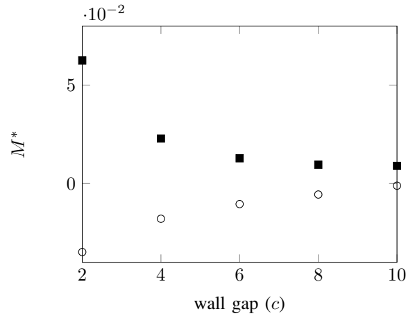
Fig. 9: Plot of moment vs wall gap (square marker: moments about y -axis; circle marker: moments about x -axis)
