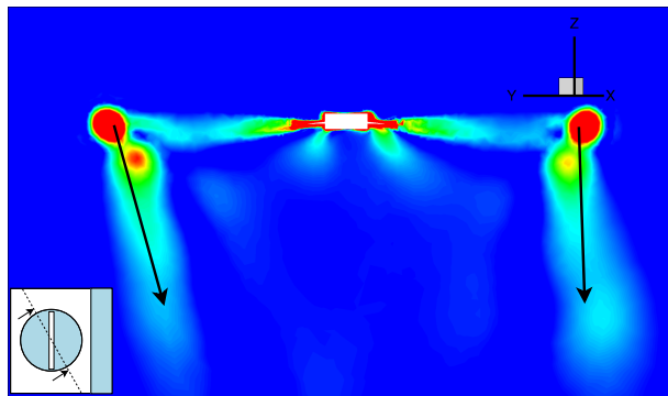
(e) Near-wall (2c gap) 60°/240° plane
