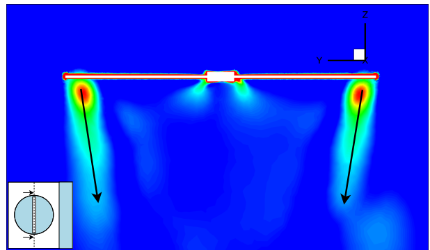
(f) Near-wall (2c gap) 90°/270° plane
