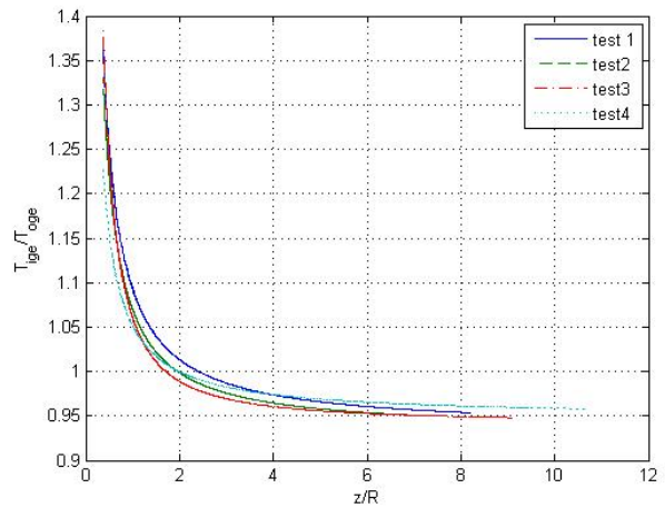
Fig. 7. Test Ground Effect vs. Empirical Ground Effect
