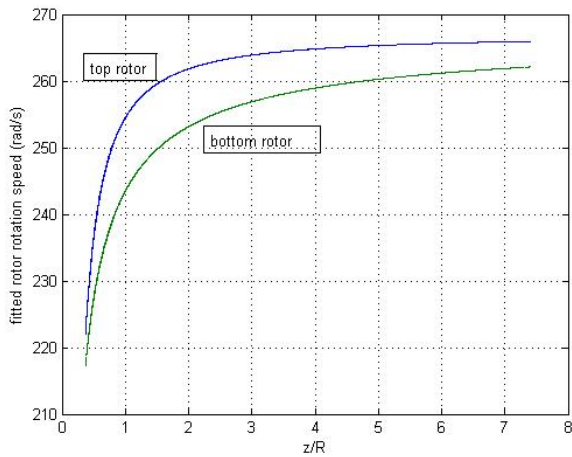
Fig. 6. Rotor speeds vs. normalized height
