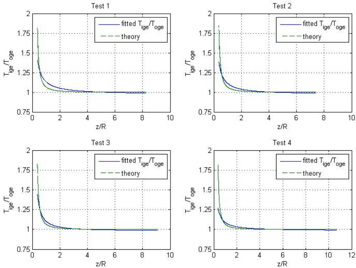
Fig. 8. Empirical GE vs. Calibrated Test GE
