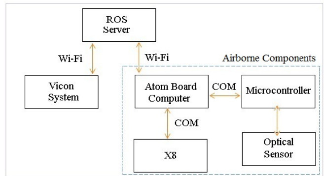
Fig. 4. Data acquisition and communication in ground effect tests
