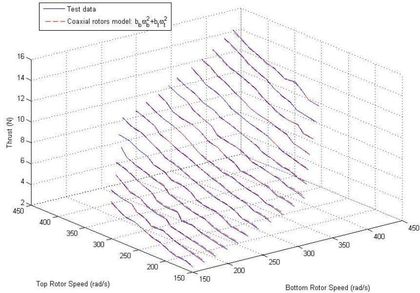
Fig. 5. Test data and fitted thrust model
