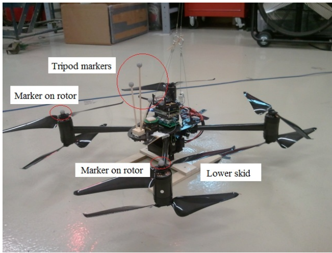
Fig. 3. X8 with lower skid and markers
