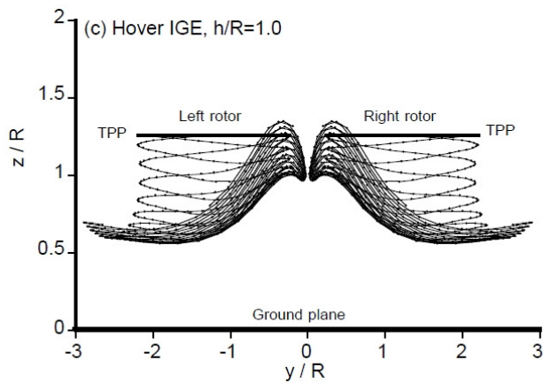
Fig. 9. Flowfield of Tandem Rotors in Ground Effect[4]
