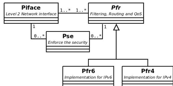
Figure 4: examples of a modular design
