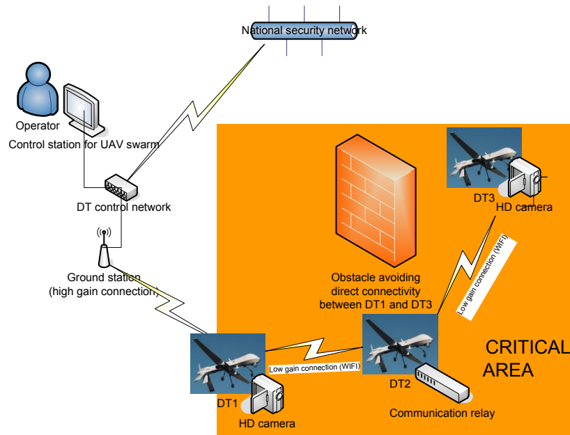
Figure 1: video surveillance use case in the SUANET project
