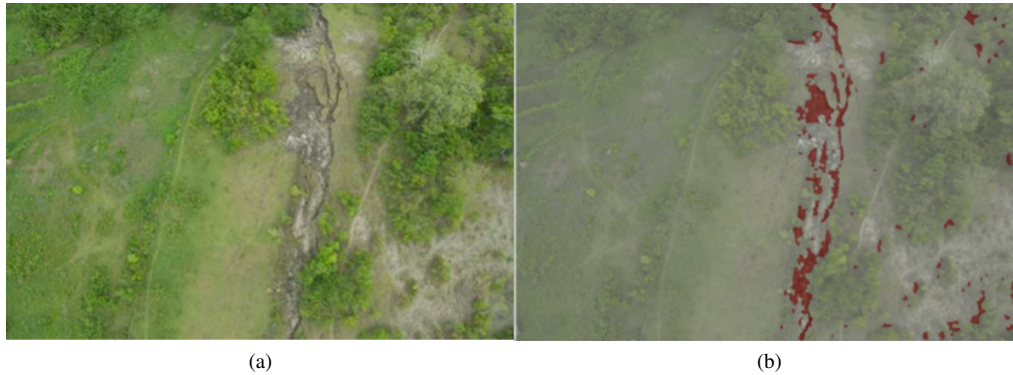
Fig. 7. Original aerial image (Fig. 7a) compared with the enhanced image (7b) of a section of the fault line discovered after the Bohol Earthquake. The fault line (highlighted red) is depicted as a vertical line near the center of the image in Fig. 7b. Some misclassified red pixels also appear in the right portion of the enhanced image.
